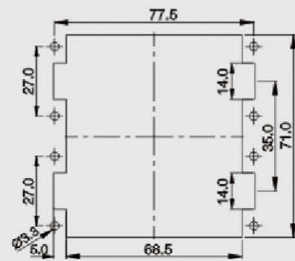
面板安装开孔图 Panel cut out
